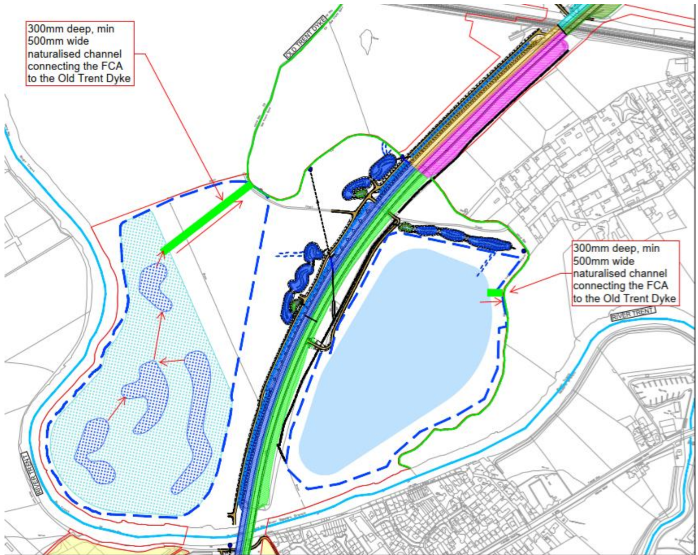
Figure 2 Option 4 indicative locations of fish escape passages from Farndon flood compensation areas into Old Trent Dyke.
